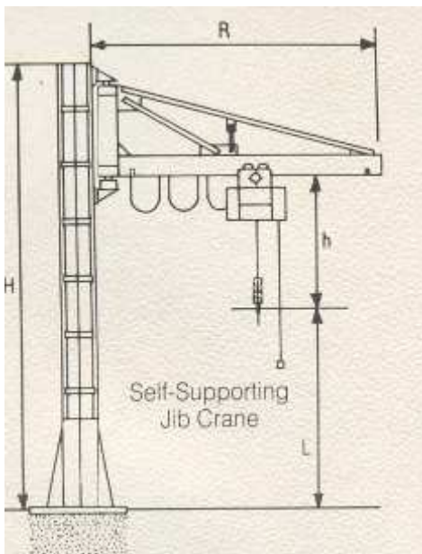
Self Supporting Jib Crane
